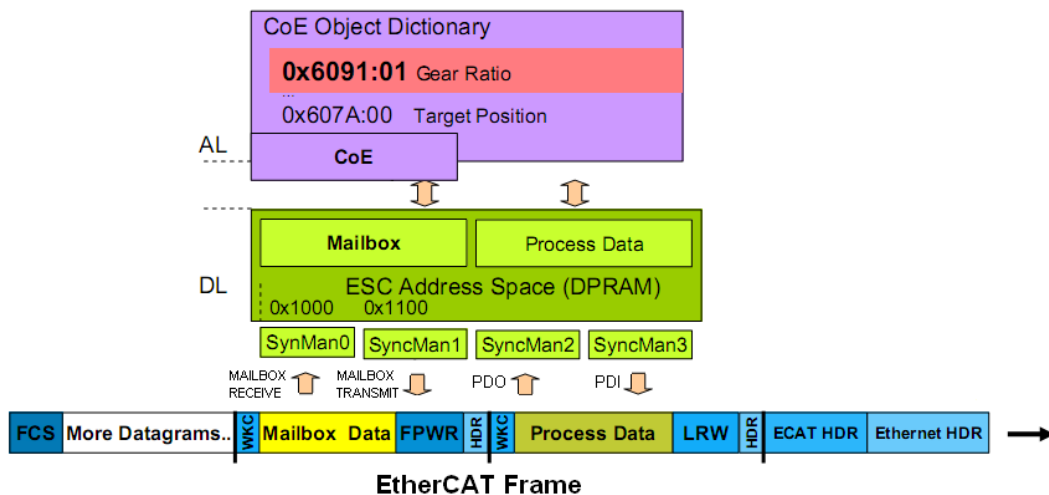
Fig. 5.1-SyncManagers assigning
